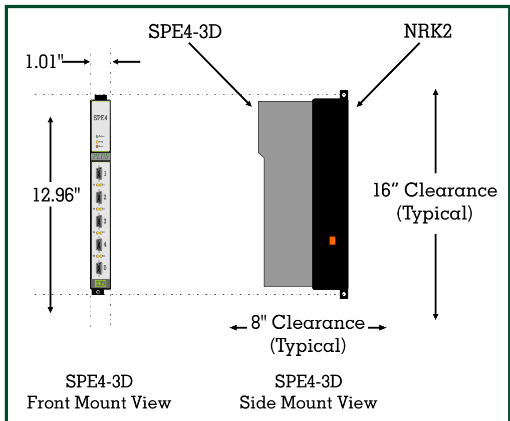
Panel Layout for SPE4-3D Installations using NRK2 Power Supply
