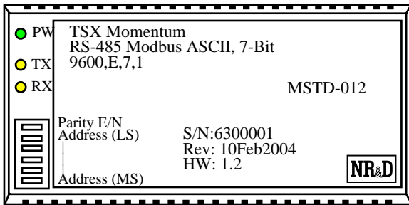
Figure 1 MSTD-012 Layout
