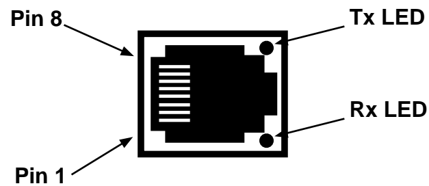
Figure 11-1 Ethernet Port RJ45
