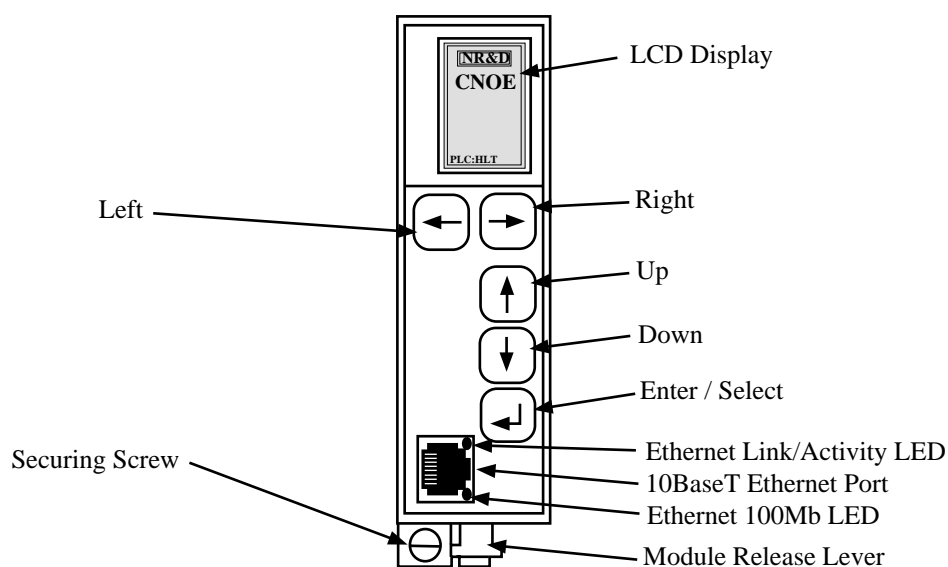
Figure 1-1 CNOE-311 Front Panel
