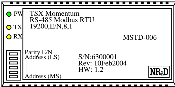
Figure 1 MSTD-006 Layout
