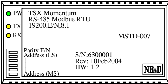
Figure 1 MSTD-007 Layout
