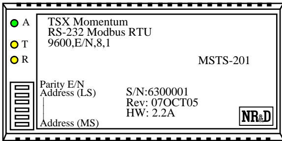
Figure 1 MSTS-201 Layout
